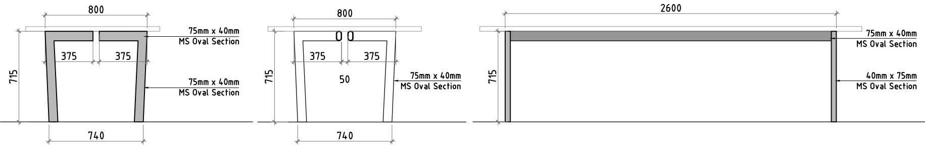
- FRONT ELEVATION
